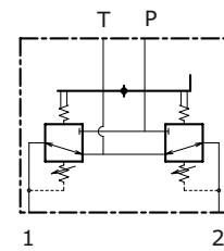
HYDRAULIC SCHEMA
