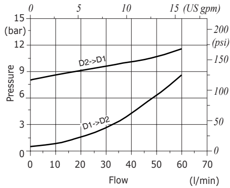
VBD 12 pressure drop vs. flow
